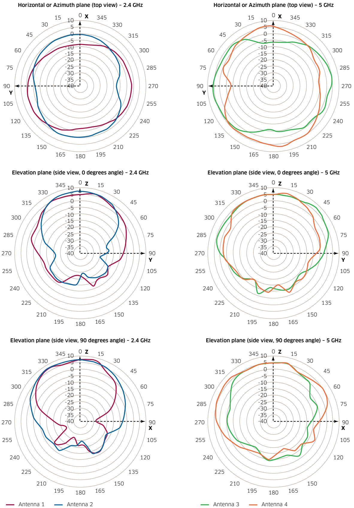
Figure 1. OmniAccess Stellar AP1251 antenna pattern plots
